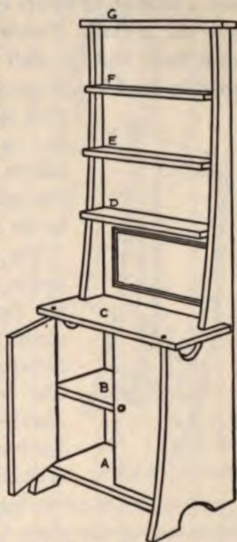
FIG. 272. — A Side-Board.
